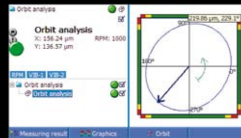
Orbit analysis
